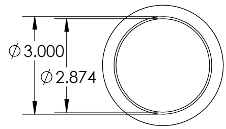
DETAIL C SCALE 1 : 3
